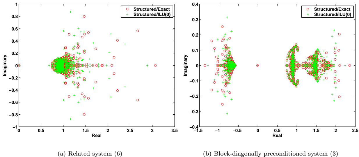
Figure 9. Eigenvalues for the related system (6) and the block-diagonally preconditioned system (3) derived from the Navier-Stokes problem with one V-cycle as splitting of the (1,1) block and approximate Schur complements using structured probing (13 vectors) with exact and ILU(0) factorizations.
