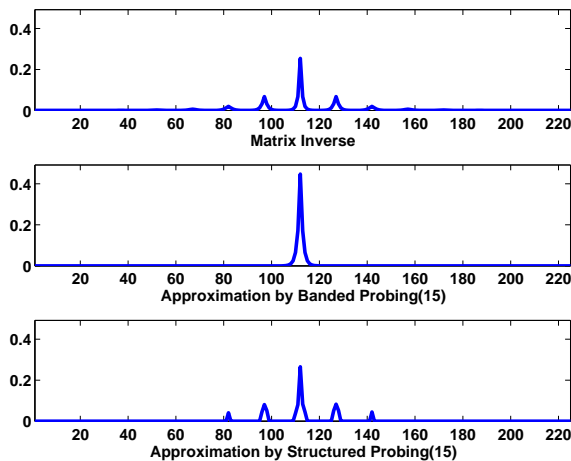
Figure 3. A typical column of the inverse of the matrix from (8) and the approximations generated by banded and structured probing with 15 vectors.
