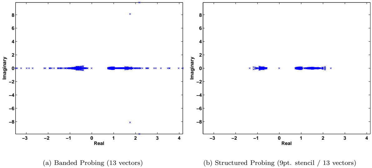
Figure 6. Eigenvalues for the block-diagonally preconditioned system (3) derived from the Navier-Stokes problem with one V-cycle as splitting of the (1,1) block and approximate Schur complements using banded and structured probing with exact factorizations.
