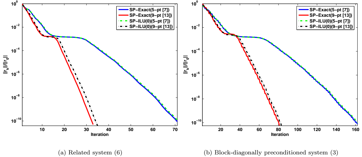
Figure 10. GMRES convergence for the Navier-Stokes problem with one V-cycle as the splitting of the (1,1) block and with an inexact Schur complement based on structured probing, using both exact and ILU(0) factorizations.
