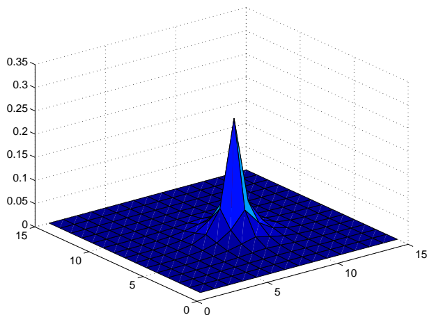
Figure 2. One column of the inverse of the matrix from (8) graphed over the underlying finite difference mesh.
