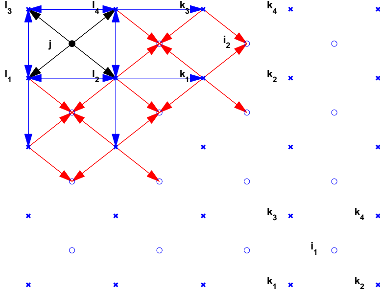
Figure 4. Entries of the Schur complement affected by node j through B^T (black arrows), F^{-1}B^T (blue arrows), assuming that the entries of F^{-1} decay sufficiently (become small) over the distance of one edge on the adjacency graph and CF^{-1}B^T (red arrows). The value |(CF^{-1}B^T)_{i_1,j}| is guaranteed to be small and |(CF^{-1}B^T)_{i_2,j}| may be large.
