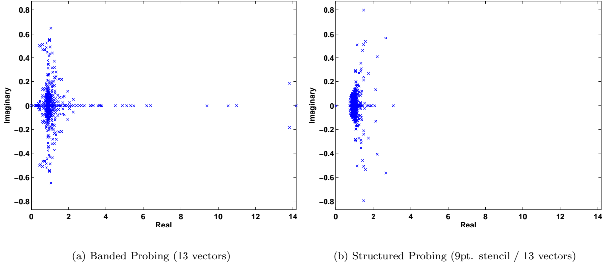
Figure 5. Eigenvalues for the related system (6) derived from the Navier-Stokes problem with one V-cycle as splitting of the (1,1) block and with approximate Schur complements from banded and structured probing with exact factorizations.
