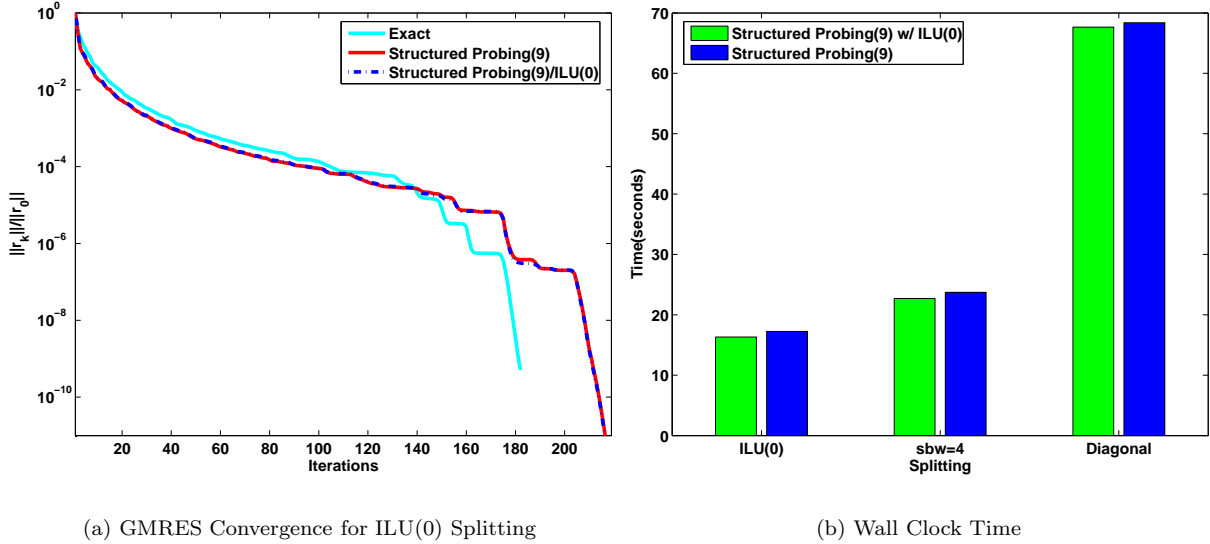
Figure 11. GMRES convergence and wall clock time for a single non-linear iteration of the metal deformation problem for various probing-based inexact Schur complements in the related system (6) and for three different splittings of the (1,1) banded matrix with semibandwidth 4, and diagonal).
