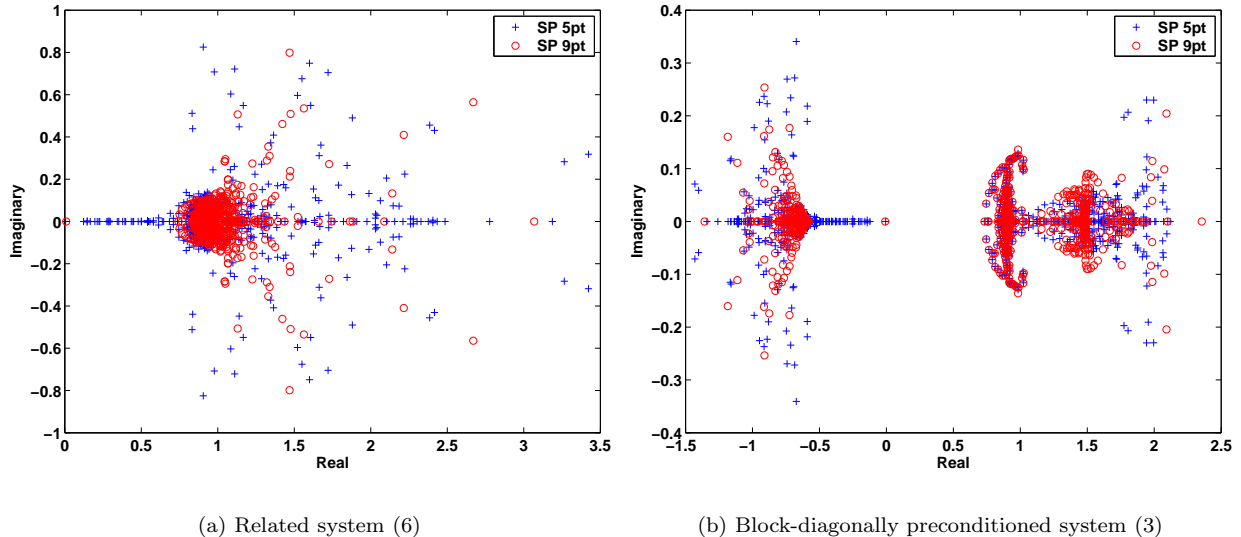
Figure 8. Eigenvalues for the related system (6) and the block-diagonally preconditioned system (3) derived from the Navier-Stokes problem with one V-cycle as splitting of the (1,1) block and approximate Schur complements using structured probing with exact factorizations.
